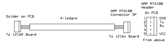
12xx Serial Interface Cable
